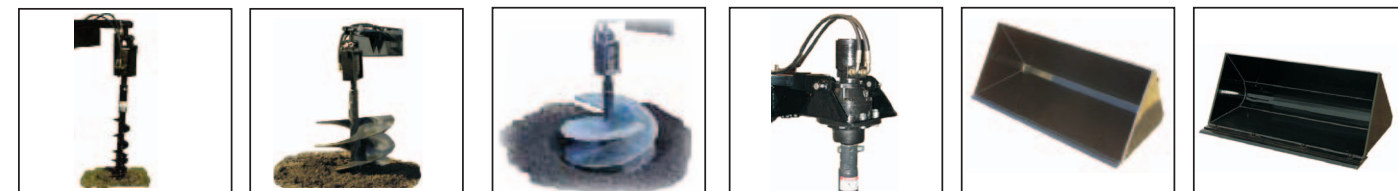
Post Hole Augers Direct drive head with 6,800 lb/in torque (peak) up to 105 RPM. Bits in 6, 9 and 12 inches. Also planetary heads. Standard Earth Augers Direct drive heads as at left. Bits in 18, 24 and 30 inches. Available with planetary heads. Tree Auger Bits in 18, 24 and 30 inch bits, designed specially for planting trees. Direct drive or planetary drive heads. Planetary Drive Power Heads with 17,600 lb/in torque (peak) - up to 60 RPM on the Ramrod 950. Material Bucket with high carbon cutting edge in 31, 36, 42 and 44 inch widths. Tooth bars available. Heavy Duty Material Bucket with replaceable cutting edge in 42 and 44 inch widths. Tooth bars available.
