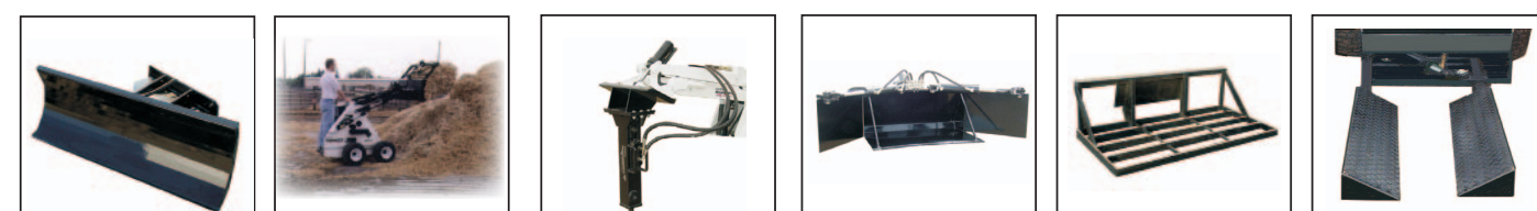
Dozer Blade Digging, backfilling, landscaping, moving snow. 48" blade with 30 degree left or right hydraulic angling. Hay and Manure Fork with Grapple - Four strong grapple tines with forks (or bucket) handle various materials. Hydraulically operated. Hydraulic Hammer - for the tough demolition work: breaker with 500 to 1,300 blows per minute at up to 184 ft. lbs. complete kit. Loose Material Handler - collects, then compresses and holds loose, sloppy type materials and debris, wood chips, some manures. Carry-all-Leveler Level loose dirt, sand etc. or transport various items. 48 by 24 inches, steel reinforced frame. Nursery Tree Tongs Hydraulic operated 36" nursery tongs, with cushion valve, to gently carry up to 24" balled trees.
